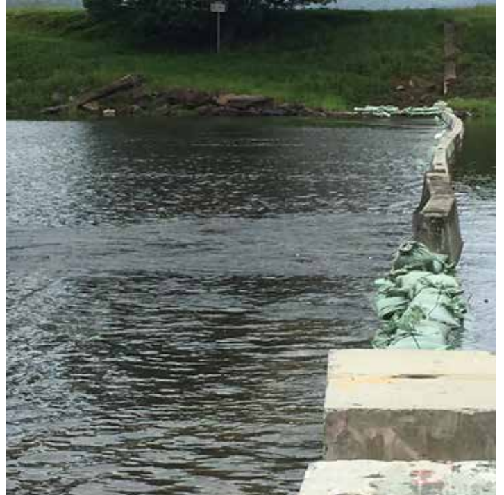
Figure 8. Tweed Shire Councils overtopping prevention controls using sandbags and concrete blocks (Source: Tweed Shire Council).
