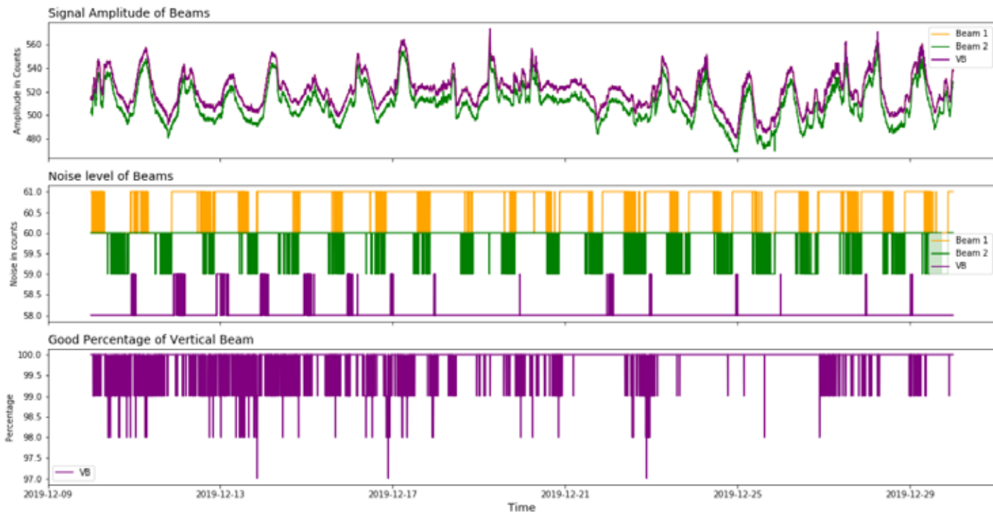
Figure 14. Signal Amplitude and Noise Levels at the RG-2-681.
