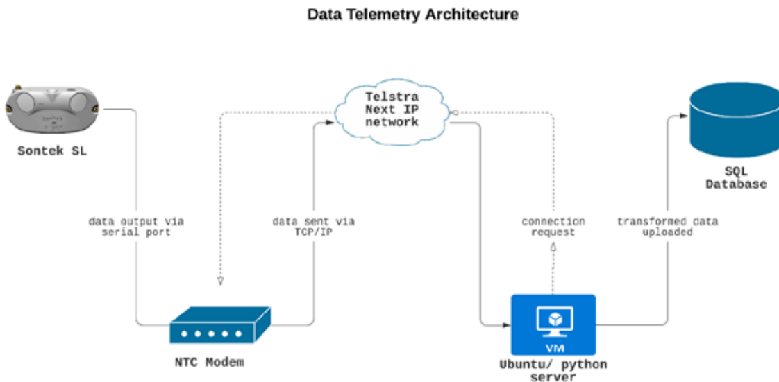
Figure 9. Flow Chart of Data Flow from the SL1500-3G (ADVIM) to MI's SQL Server.
