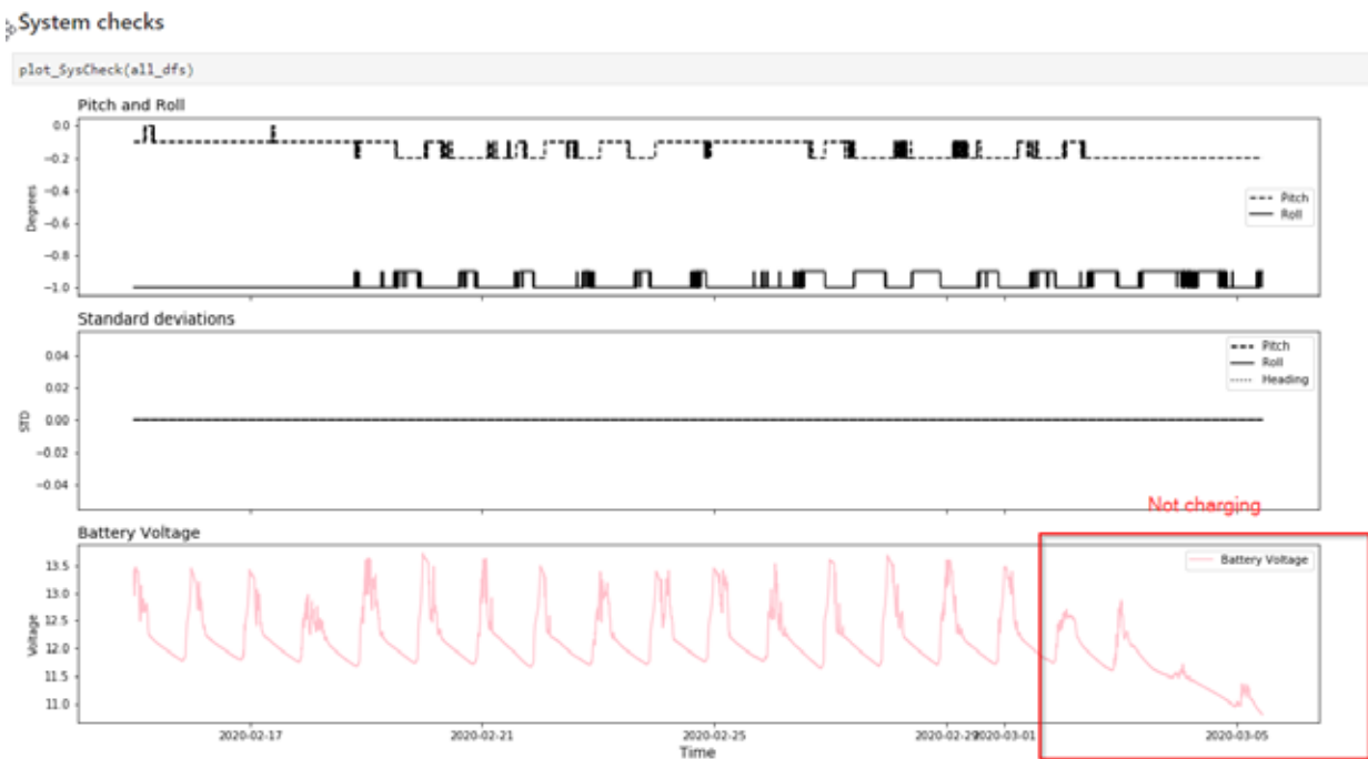
Figure 13. Pitch/Roll and Battery Voltage Plots.
