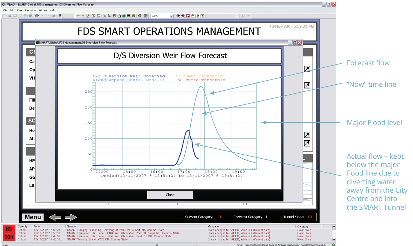
Figure 4. Model and actual flow curves – note the forecast and now time line, the moderate and major flood levels and the flow curve showing the effectiveness of diverting the water away from the City into the Tunnel.
