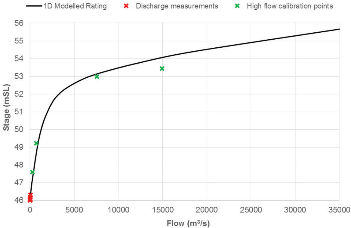
Figure 8: Calibrated 1D modelled stage-flow rating.
