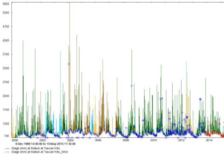
Figure 7: Water Level data from a Horizons Regional Council site (Makuri at Tuscan Hills) quality coded to the NEMS Water Level measurement standard. Blue diamonds represent on site verification of the data that is one of the components used to quality code the data.
