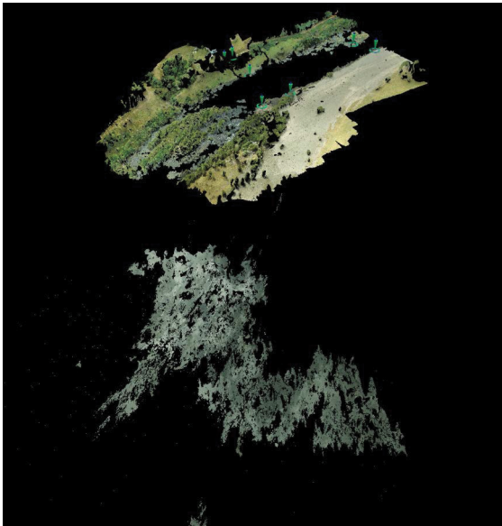
Figure 4: Pre-processing of point cloud showing terrain model with superfluous data interpolated by cloud reflections on water surface.
